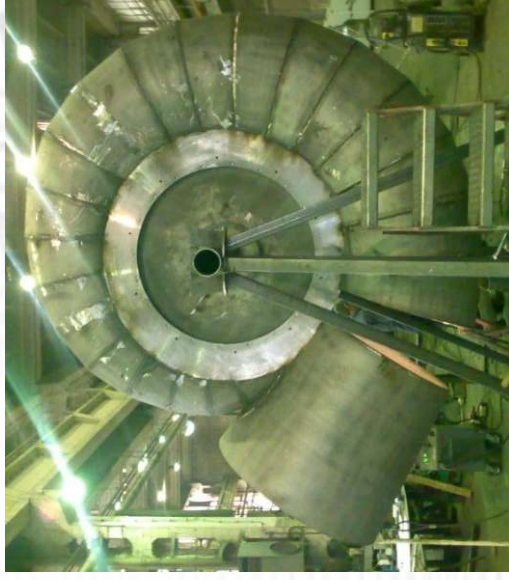
Spiral case of water turbin (d. 4,5 m)
